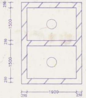
DETL. OF UNDER GROUND WATER RESERVIOR(U.G.R.)
