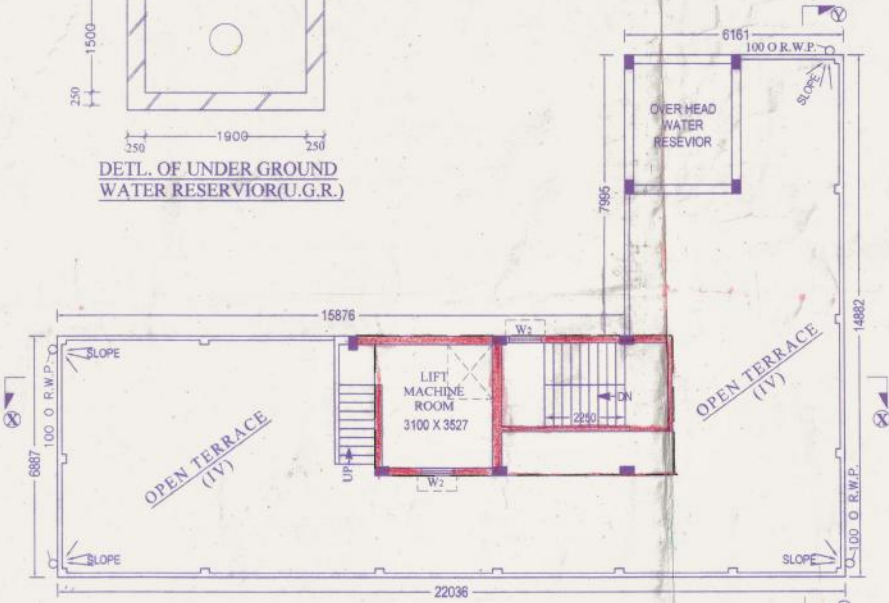
TERRACE PLAN
