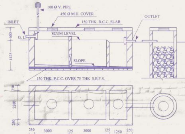
DETL. OF SEPTICTANK & SOAK PIT (FOR 100 USER)
