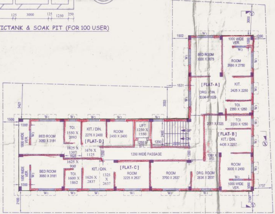
TYPICAL FLOOR PLAN (FIRST, SECOND & THIRD)
